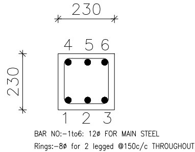
LINTEL BEAM LB2
