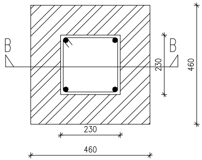
PLAN OF COLUMN BC-1(460x460) BAR NO:- 1T04-16Ø RINGS:-8@150c/c THROUGHOUT
