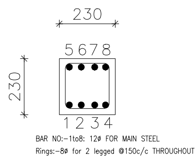
LINTEL BEAM LB1
