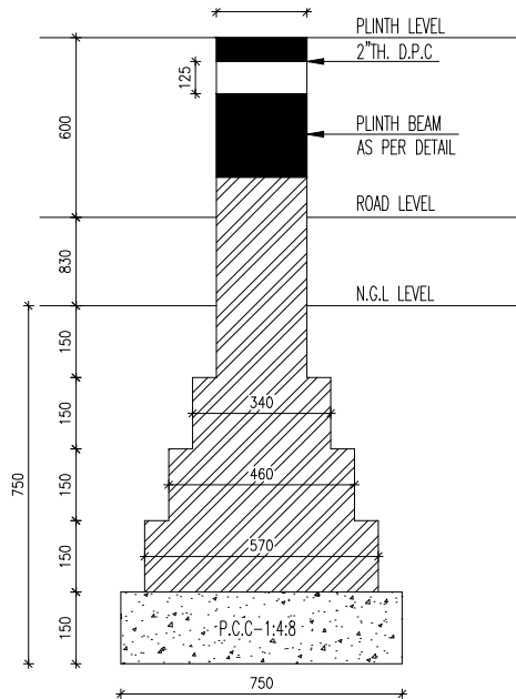
FOUNDATION OF 230 TH. BRICK WALL(FW1)
