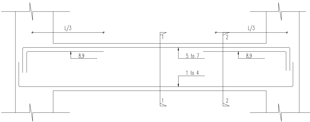
L-SEC OF BEAM B-1
