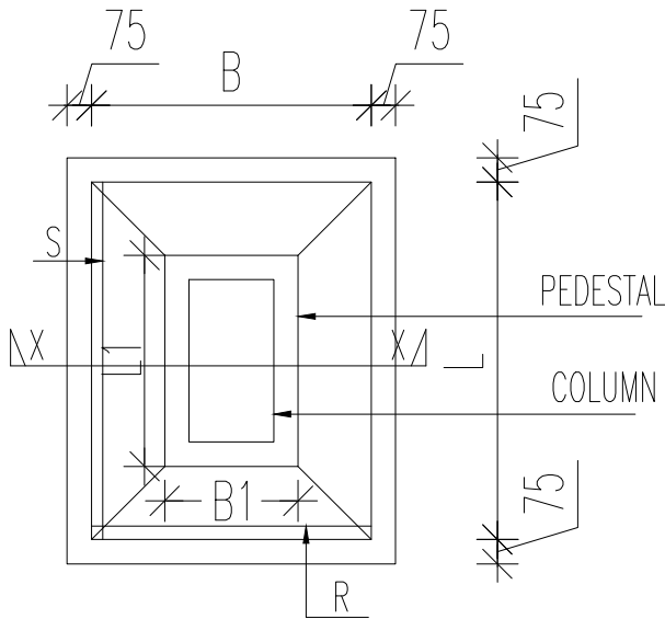
TYPICAL PLAN OF COLUMN FOOTING
